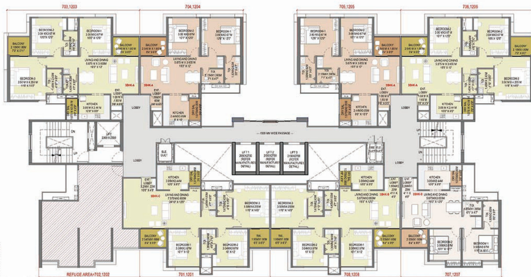
BUILDING A- REFUGE FLOOR
